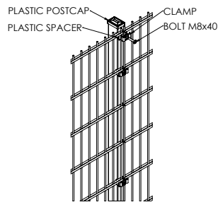
DETAIL ASSEMBLY INTERMEDIATE POST
