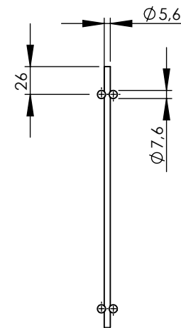
DETAIL B SCALE 1 : 5
